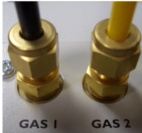
Figure 2-8: Gases connected to GDUnet
