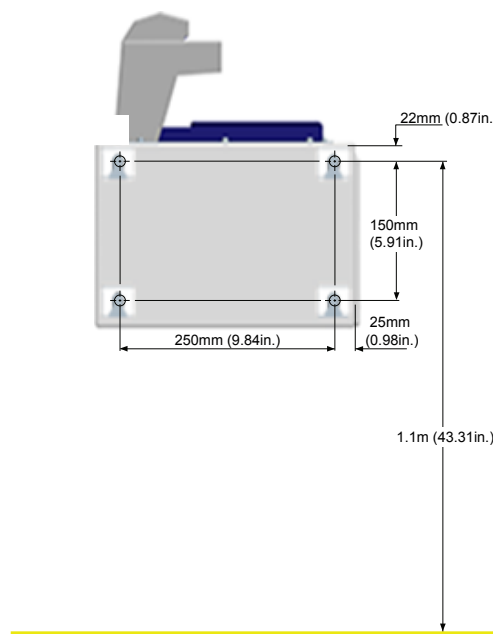
Figure 2-1: Wall Mounting Dimensions
