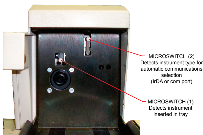
Figure 3-5: Microswitches
