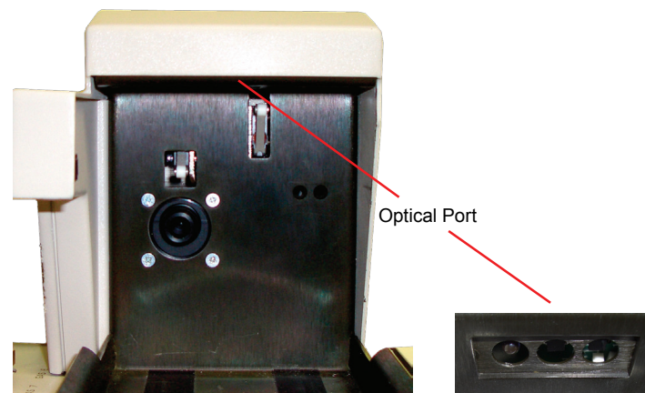
Figure 3-3: Optical port
