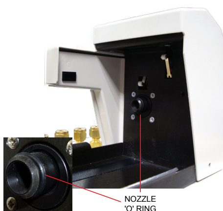
Figure 3-6: Gas outlet nozzle
