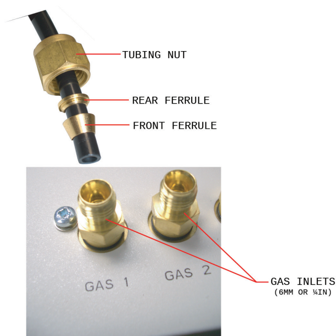
Figure 2-7: Tubing Nut / Ferrules Setup
