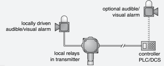
LOCALLY DRIVEN ALARM SYSTEM
