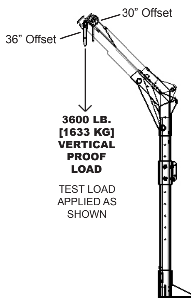
Figure #5.1c: DK3036 with/ 30" Offset & 36" Offset
