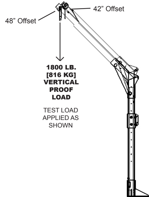
Figure #5.1d: DK4248 with/ 42" Offset & 48" Offset
