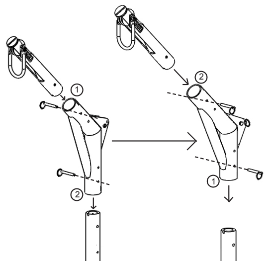
Figure #5.2e: DK Series Davit Elbow Reversible for longer offset
