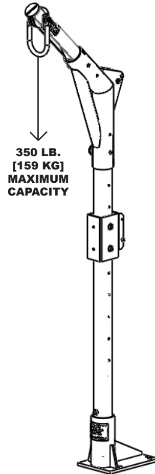
Figure #5.1a: DK Series Davit shown with DS Series Floor Mount
