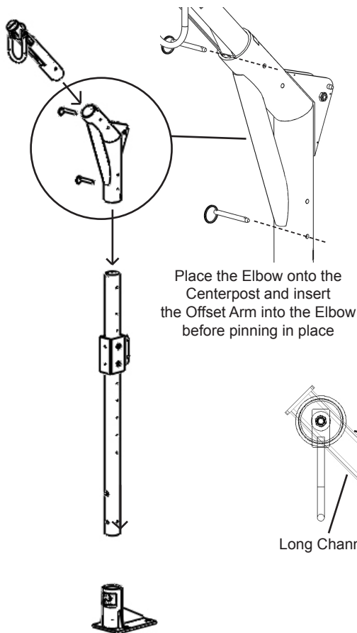
Figure #5.2b: DK Series Davit with/ DS Series Sleeve Installation
