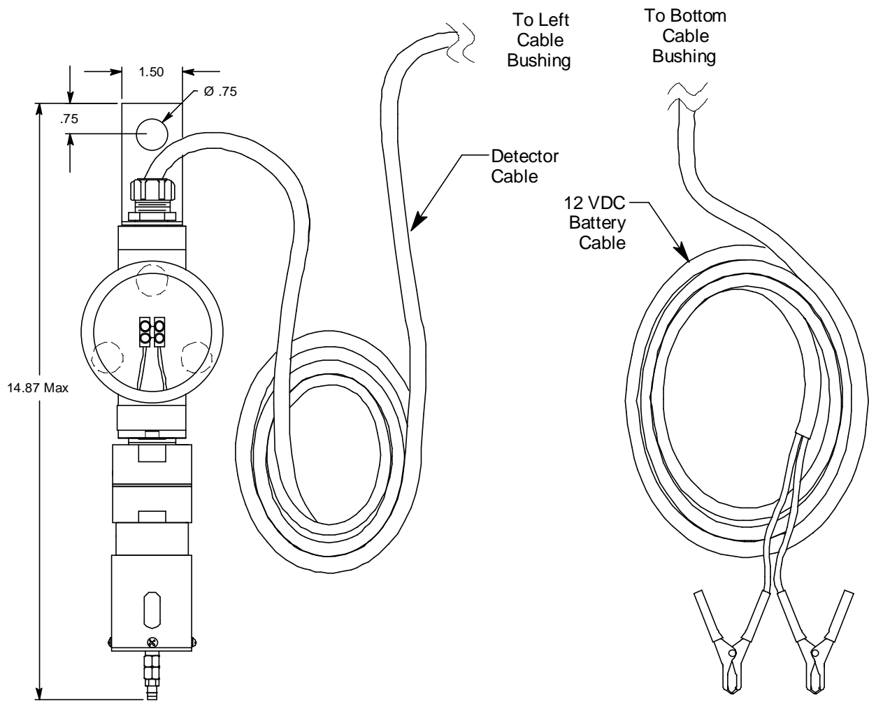
Figure 7: H 2 S Junction Box Outline & Mounting Dimensions
