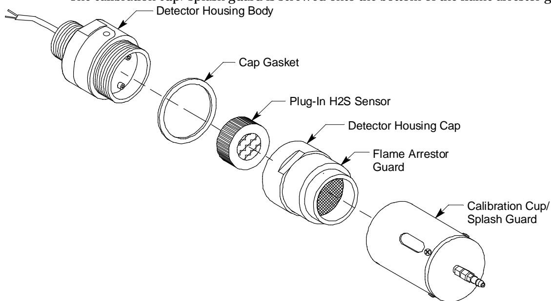
Figure 3: H 2 S Detector Component Location
