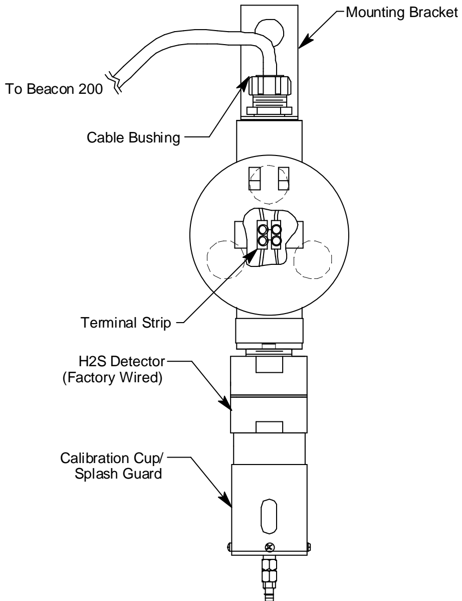
Figure 2. H 2 S Junction Box Component Location
