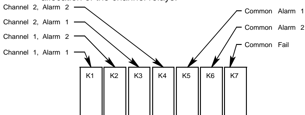
Figure 5. Beacon 200 Rig Monitor Channel Relay Allocation
