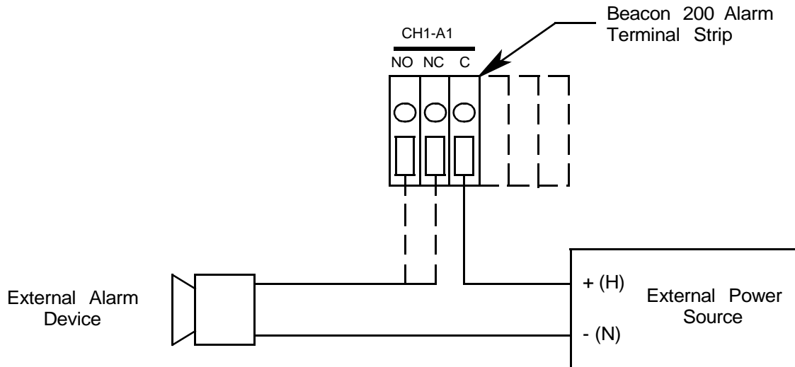
Figure 9. Typical External Alarm Wiring
