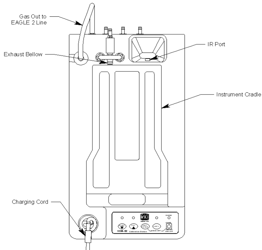
Figure 6: Instrument Panel
