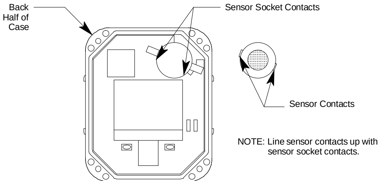
Figure 16: Replacing the Sensor
