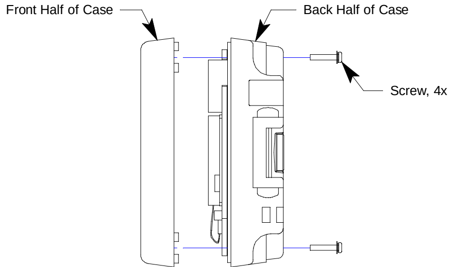
Figure 15: Case Separation
