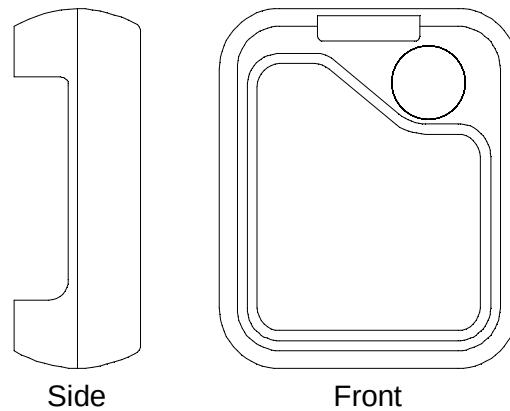
Figure 2: Rubber Boot
