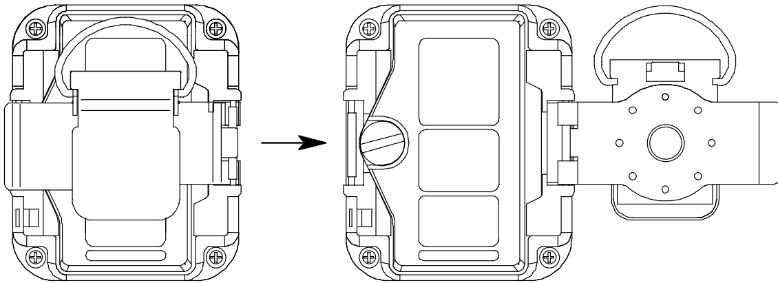
Figure 13: Clip Release
