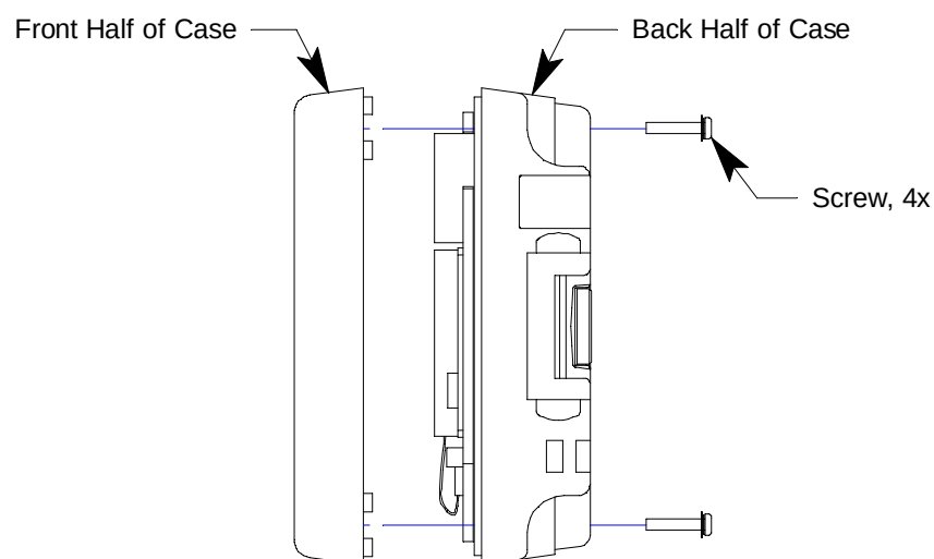
Figure 17: Case Separation
