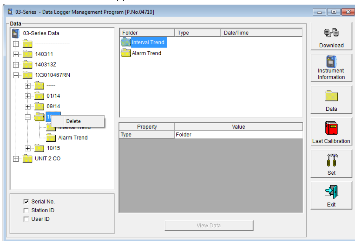
Figure 48: Delete Box
