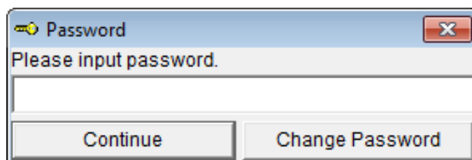
Figure 49: Password Window
