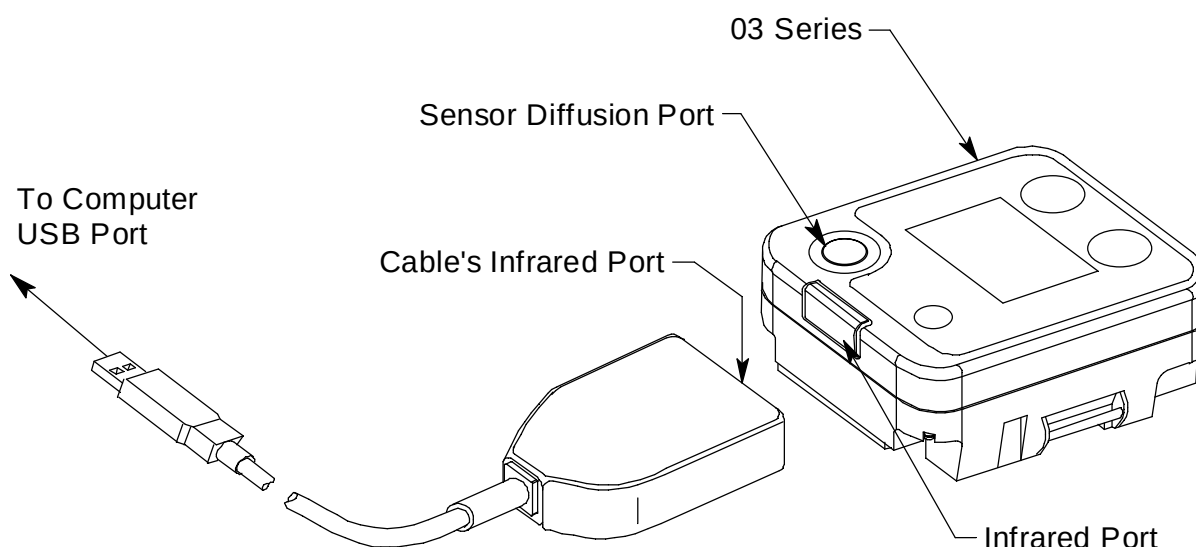
Figure 14: Aligning the 03 Series with the Cable Infrared Receiver
