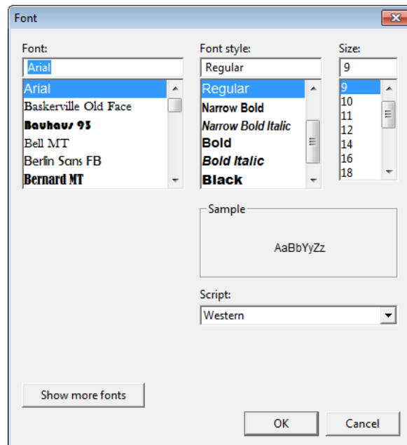
Figure 67: Font Window
