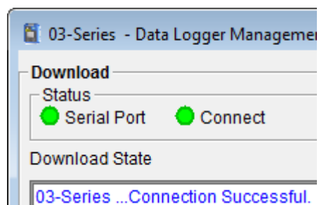
Figure 15: Connection Message
