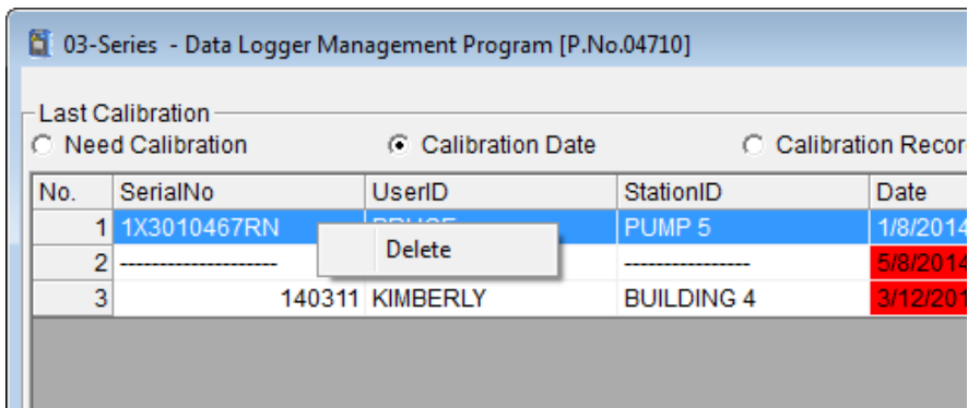
Figure 61: Delete Box
