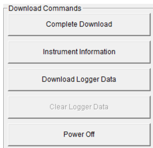
Figure 16: Download Commands
