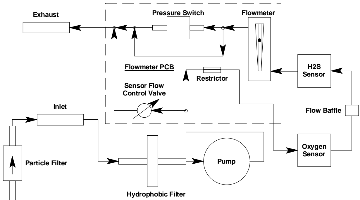
Figure 2: Oxygen/Hydrogen Sulfide Sample-Draw Detector Flow Diagram
